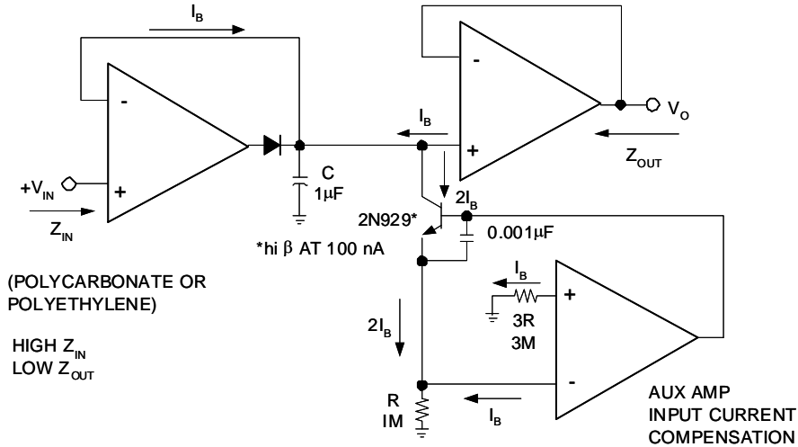
Low Drift Peak Detector
