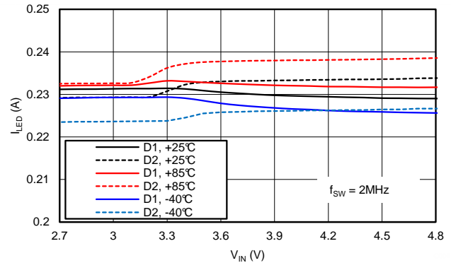
Figure 16. Torch Current Line Regulation
