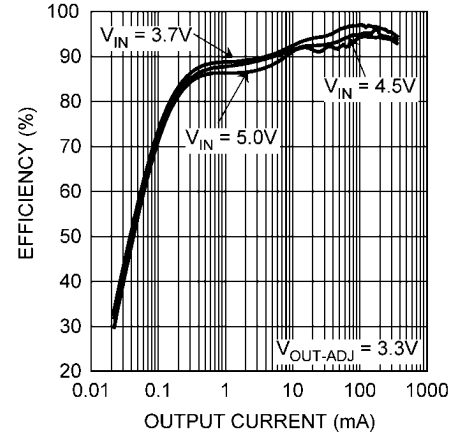
Efficiency vs. Output Current ( V_{OUT-ADJ} = 3.3V , L = 2.2 \mu H , dcr = 200m\Omega )
