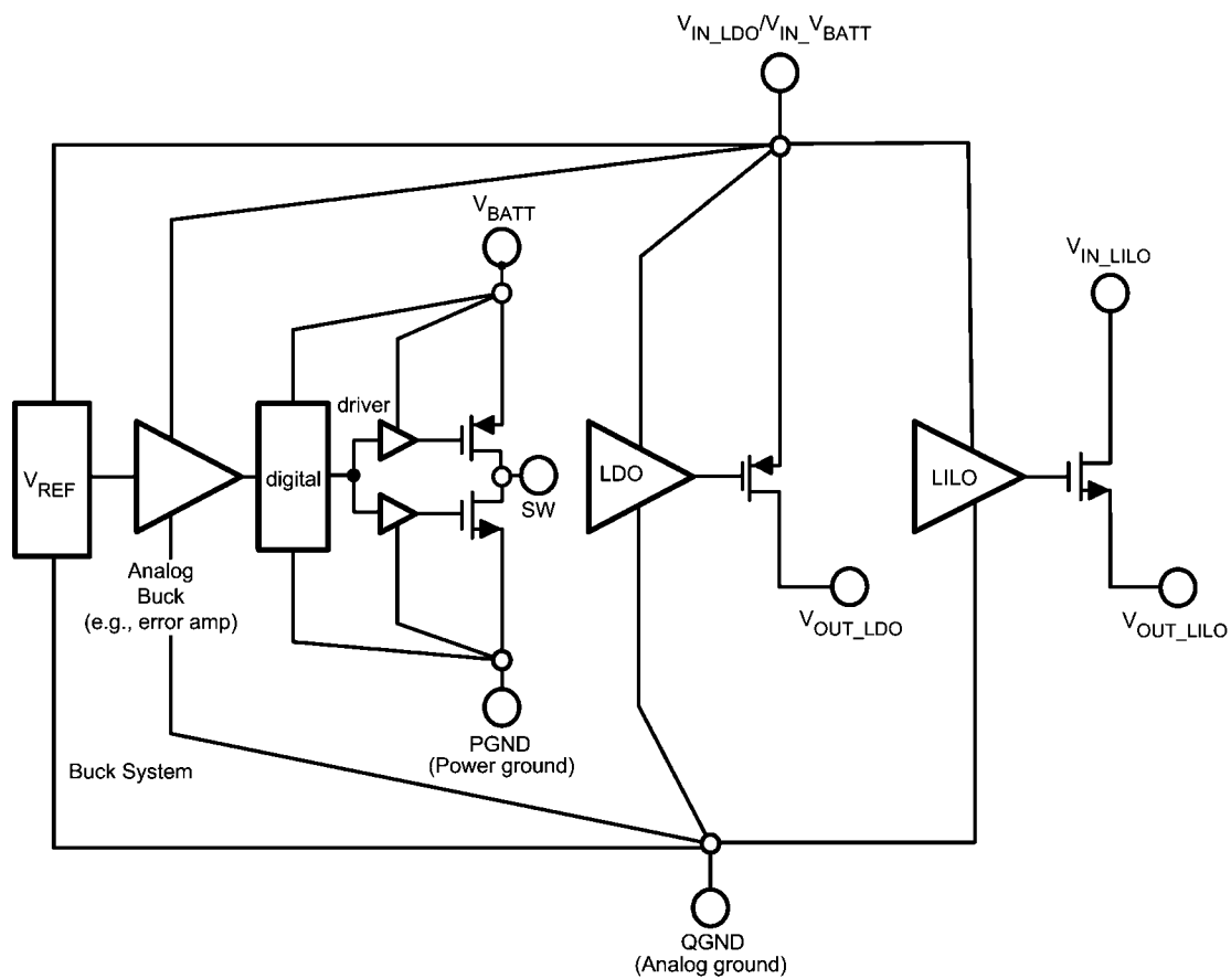
FIGURE 2. Functional Diagram (Always Connecnt VIN_LDO to VBATT)
