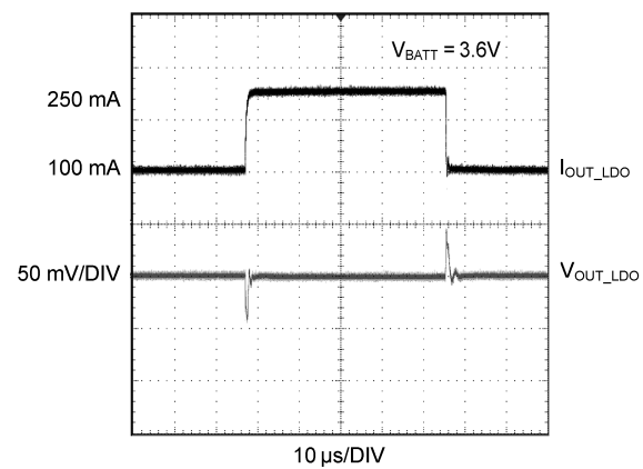
Load Transient Response LDO 100mA to 250mA
