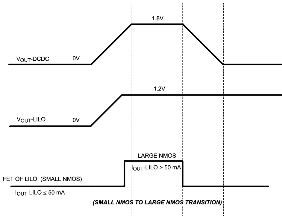
FIGURE 3. Mode Transition
