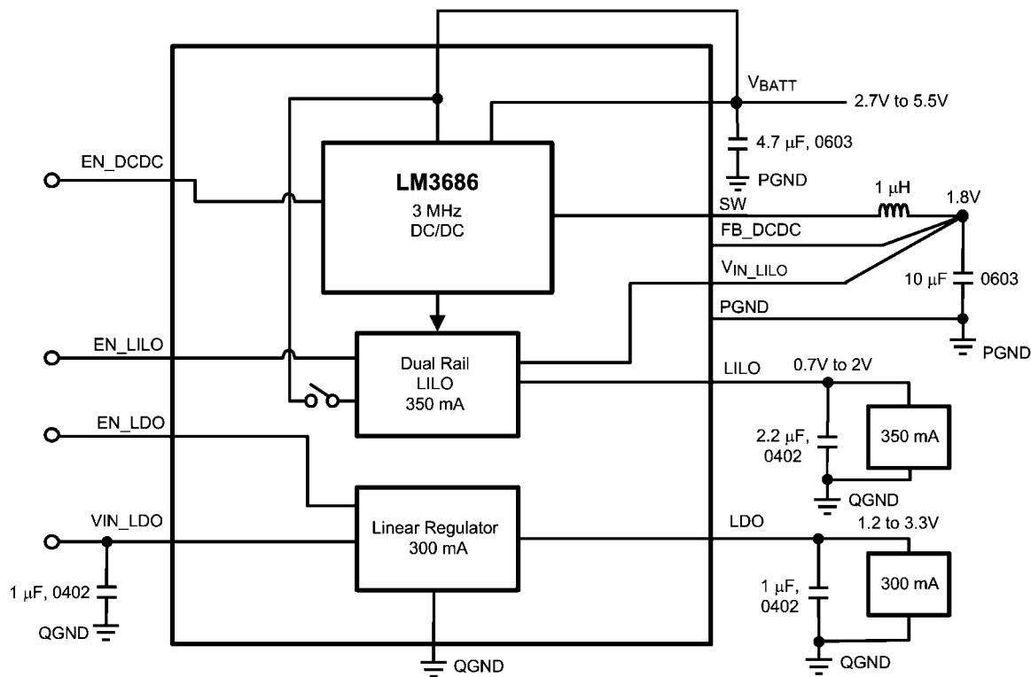
FIGURE 1. Typical Application
