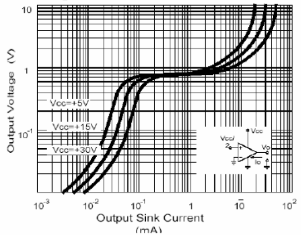
Fig.10 Output Characteristics Current sinking
