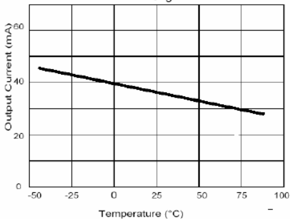
Fig.11 Current Limiting
