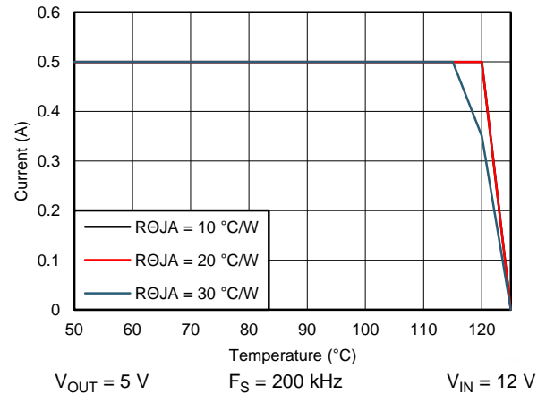
Figure 70. Derating Curve
