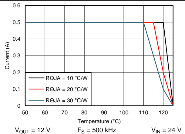
Figure 88. Derating Curve
