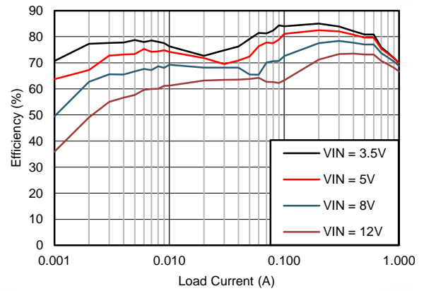
Figure 48. Efficiency
