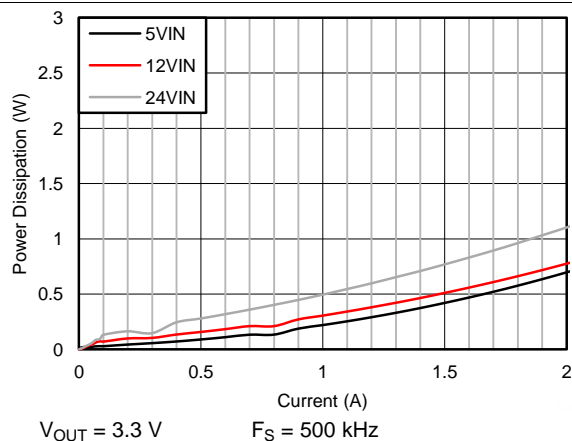
Figure 43. Power Loss at Room Temperature
