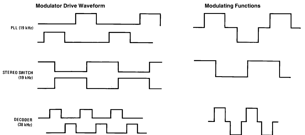
FIGURE 3. Digital Waveforms
