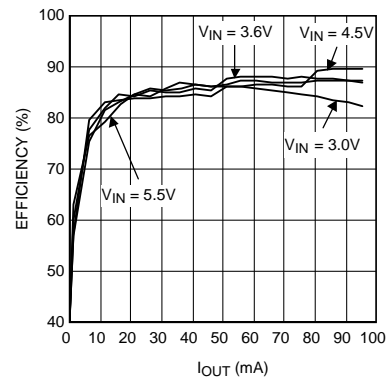
Figure 21. Efficiency vs Output Current ( V_{OUT} = 12\text{ V} )
