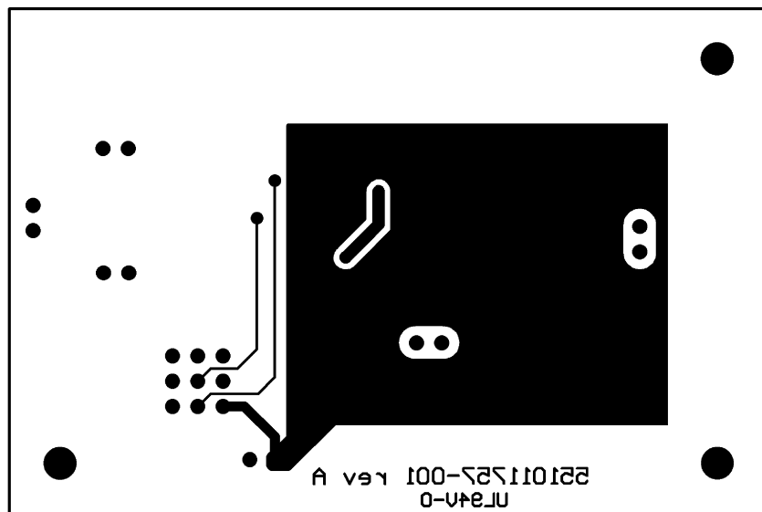
Figure 43. Bottom Layer
