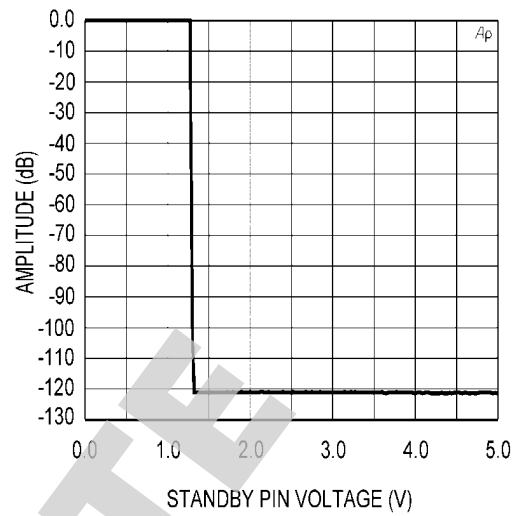
Standby Attenuation vs Standby Pin Voltage ±17V, P_O = 1W , R_L = 8\Omega , 80kHz BW
