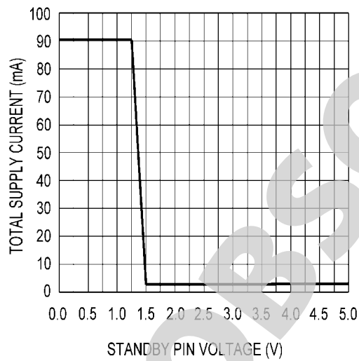
Supply Current vs Standby Pin Voltage ±17V
