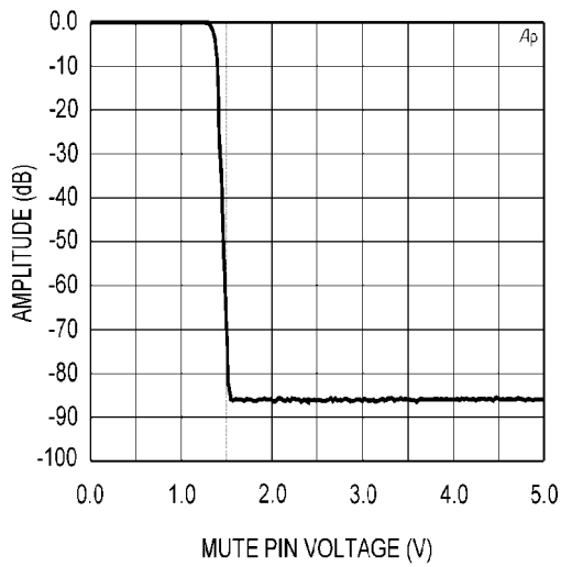
Mute Attenuation vs Mute Pin Voltage ±17V, P_O = 1W , R_L = 8\Omega , 80kHz BW
