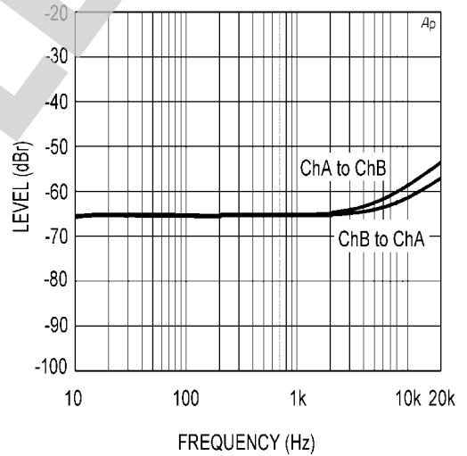
Crosstalk vs Frequency \pm 17V , P_O = 10W , R_L = 8\Omega , 80kHz BW
