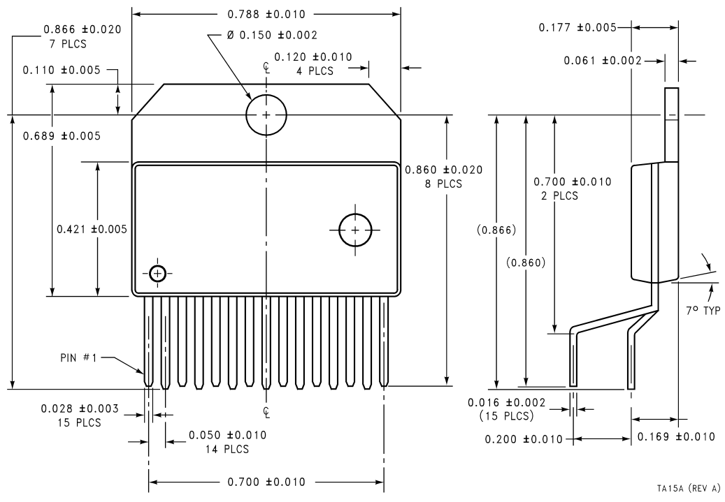
Staggered Lead Non-Isolated Package NS Package Number TA15A
