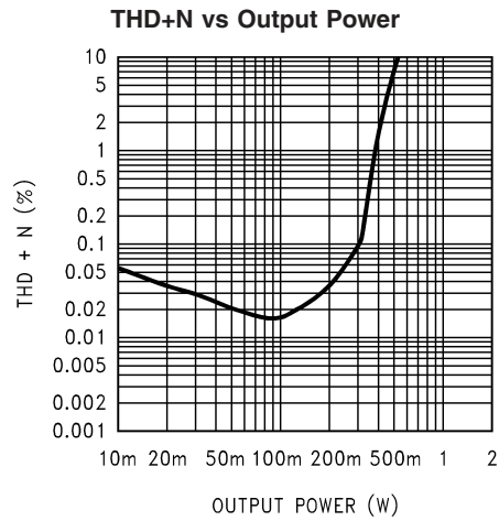
20073628 V_{DD} = 3V, R_L = 8\Omega, f_{IN} = 1kHz
