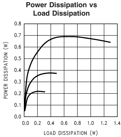
20073634 V_{DD} = 5\text{V} , f_{IN} = 1\text{kHz} , at (from top to bottom at 0.2W): R_L = 8\Omega , R_L = 16\Omega , R_L = 32\Omega
