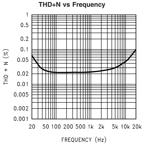
20073624 V_{DD} = 5V, R_L = 8\Omega, P_{OUT} = 150mW
