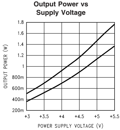
20073602 R_L = 8\Omega , f_{IN} = 1\text{kHz} , at (from top to bottom at 4.5V): THD+N = 10%, THD+N = 1%
