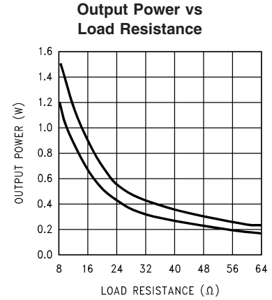
20073637 R_L = 8\Omega , f_{IN} = 1\text{kHz} , at (from top to bottom at 24Ω): THD+N = 10%, THD+N = 1%
