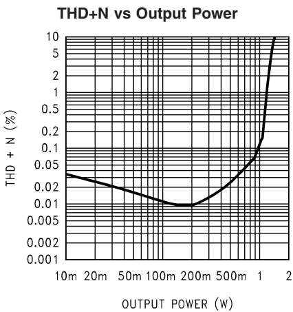
20073633 V_{DD} = 5V, R_L = 8\Omega, f_{IN} = 1kHz
