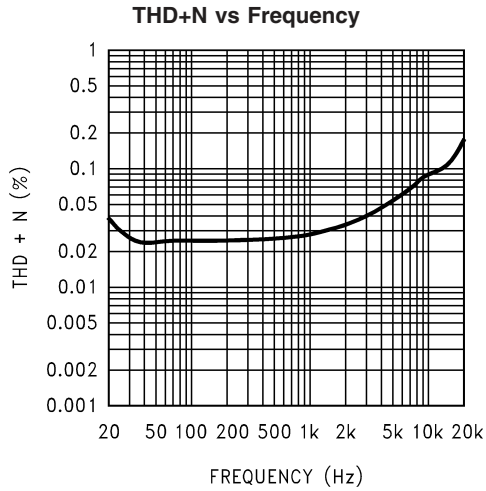
20073617 V_{DD} = 3V, R_L = 8\Omega, P_{OUT} = 150mW
