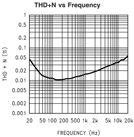
20073620 V_{DD} = 5.5V, R_L = 8\Omega, P_{OUT} = 150mW
