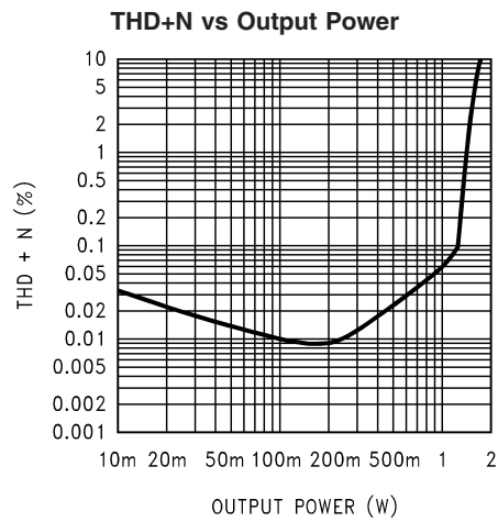
20073630 V_{DD} = 5.5V, R_L = 8\Omega, f_{IN} = 1kHz
