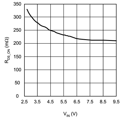
R_{DS(ON)} ( ON ) vs V_{DD}
