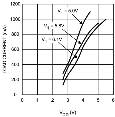
Load Current vs V_{DD} Z_L = 2\mu F + 30\Omega
