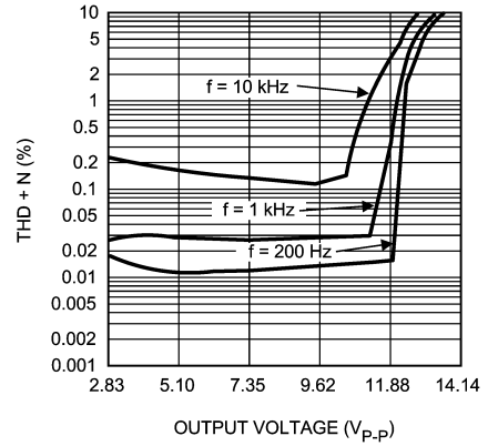
THD+N vs Output Voltage V_{DD} = 4.2V, Z_L = 2\mu F + 30\Omega, V_1 = 6.1V
