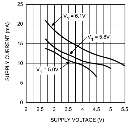
Supply Voltage vs Supply Current Z_L = 2\mu F + 30\Omega, V_{IN} = 0V
