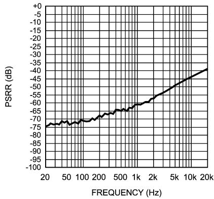
PSRR vs Frequency V_1 = 5.0V, Z_L = 2\mu F + 30\Omega, V_{ripple} = 200mV_{pp}, A_{V-BTL} = 26dB
