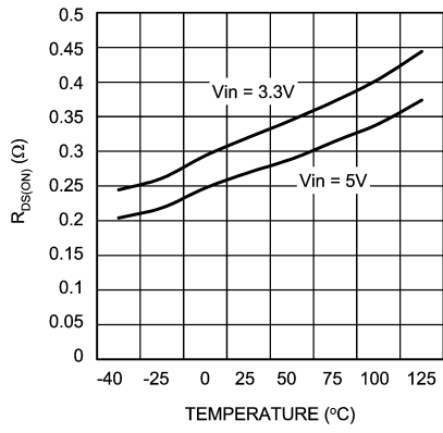
R_{DS(ON)} ( ON ) vs Temperature
