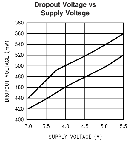
R_L = 8\Omega, f_{IN} = 1kHz , at (from top to bottom at 4.5V): positive signal swing, negative signal swing
