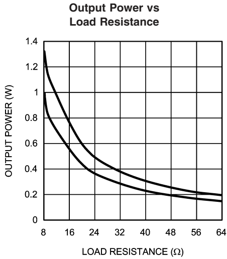
V_{DD} = 5V, f_{IN} = 1kHz , at (from top to bottom at 32 \Omega ): THD+N = 10%, THD+N = 1%
