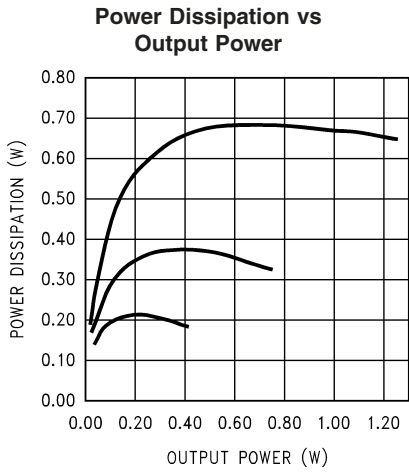
V_{DD} = 5V, f_{IN} = 1kHz , at (from top to bottom at 0.20W): R_L = 8\Omega, 16\Omega, 32\Omega
