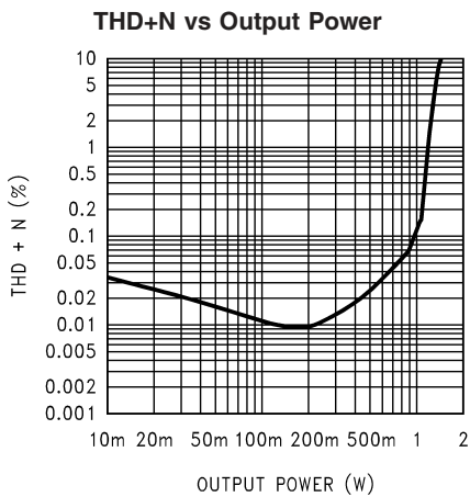
20078133 V_{DD} = 5V, R_L = 8\Omega, f_{IN} = 1kHz
