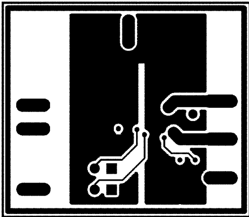
FIGURE 11. Layer 2 (GND)
