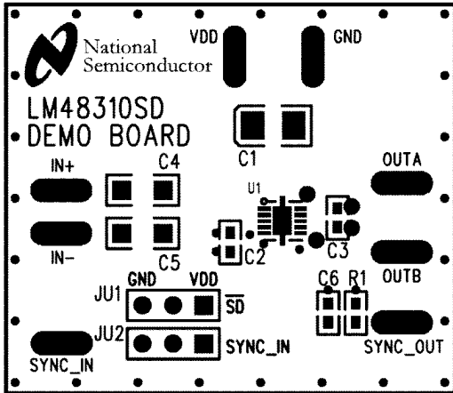
FIGURE 9. Top Silkscreen
