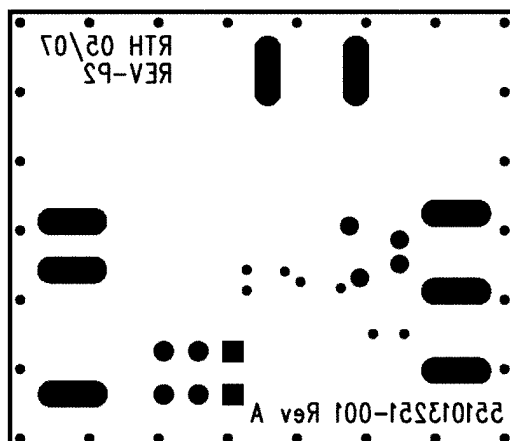
FIGURE 14. Bottom Silkscreen
