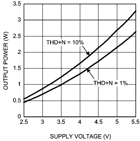
www.DataSheet4U.com Output Power vs Supply Voltage f = 1\text{kHz}, R_L = 4\Omega
