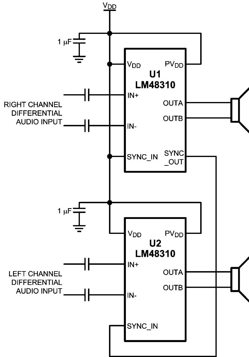
FIGURE 2. Cascaded LM48310
