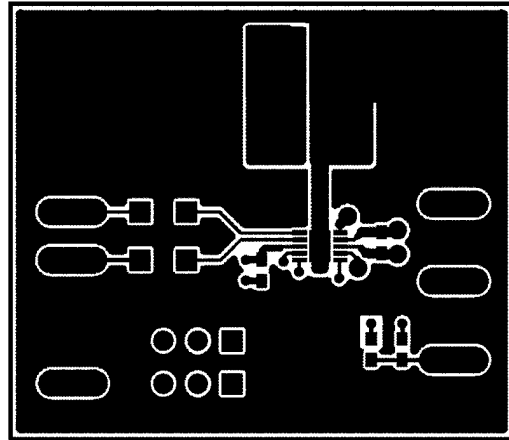
FIGURE 10. Top Layer
