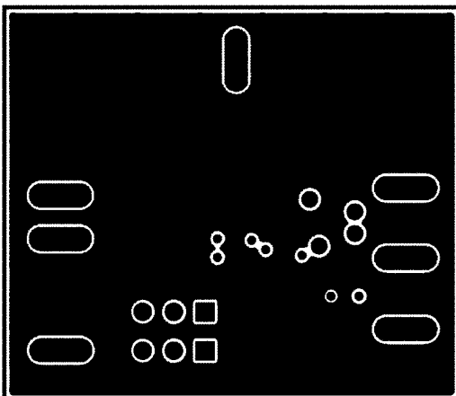
FIGURE 13. Bottom Layer
