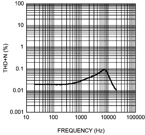
www.DataSheet4U.com THD+N vs Frequency V_{DD} = 3.6V, P_O = 1.25W, R_L = 3\Omega
