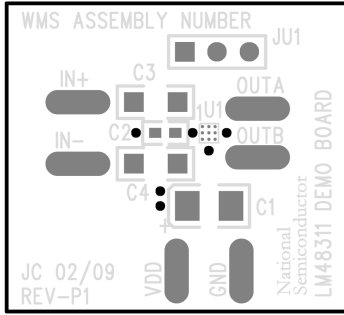
FIGURE 7. Top Silkscreen 30097526
