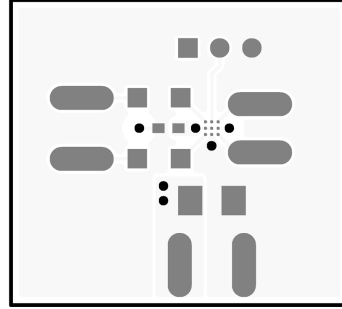
FIGURE 8. Top Layer 30097525
