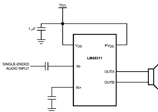
FIGURE 5. Single-Ended Input Configuration
