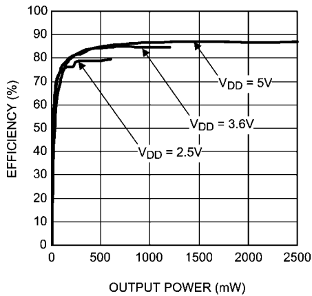
Efficiency vs Output Power f = 1kHz, R_L = 4\Omega
