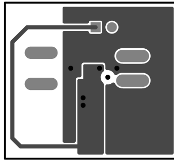
FIGURE 10. Bottom Layer 30097523
