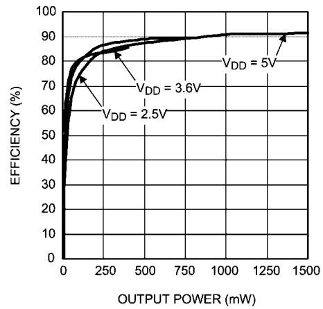
Efficiency vs Output Power f = 1kHz, R_L = 8\Omega
