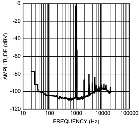
www.DataSheet4U.com Spread Spectrum Output Spectrum vs Frequency V_{DD} = 5.0V, V_{IN} = 1V_{RMS}, R_L = 8\Omega
