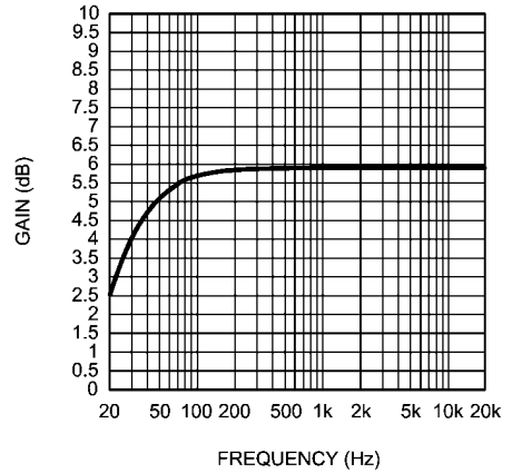
LM4844TL Frequency Response V_{DD} = 5V, R_L = 32\Omega , Mode 9 HP, Full Gain = 6dB
