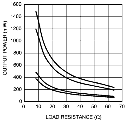
LM4844TL Output Power vs Load Resistance, LS Top- V_{DD} = 5V, 10\% THD+N ; Topmid- V_{DD} = 5V, 1\% THD+N Botmid- V_{DD} = 3V, 10\% THD+N ; Bot- V_{DD} = 3V, 1\% THD+N
