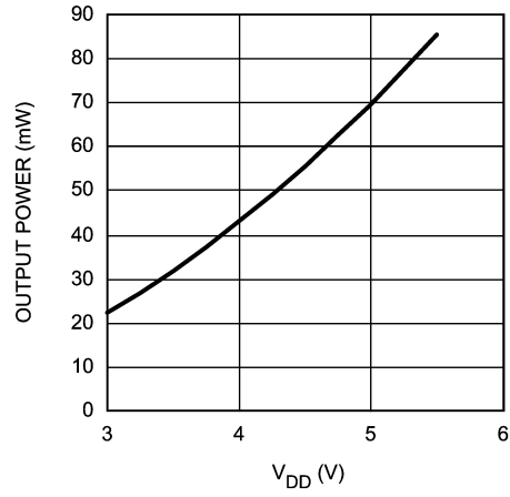
Output Power vs Supply Voltage R_L = 32\Omega , SE, Mode 4
