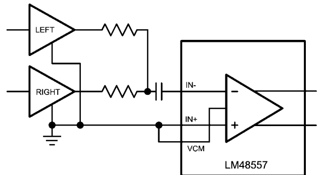
Inverting Configuration
