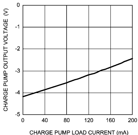
Charge Pump Output Voltage vs Load Current V_{DD} = 4.2V
