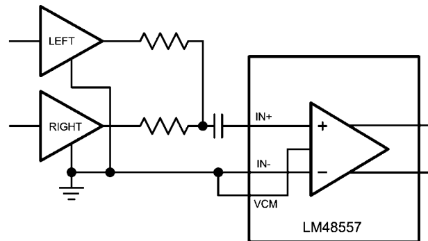
Non-Inverting Configuration
