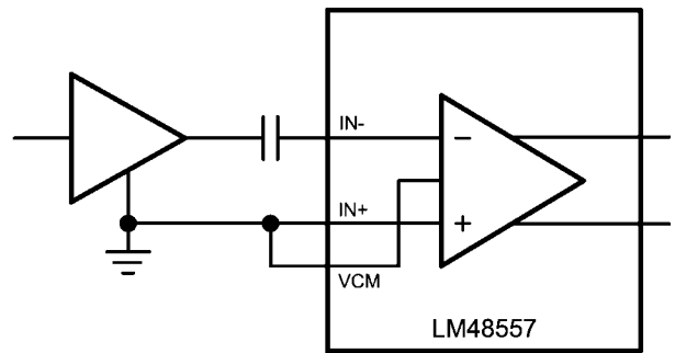
Inverting Configuration
