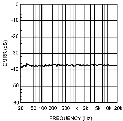
www.DataSheet4U.com CMRR vs Frequency V_{DD} = 4.2V , V_{RIPPLE} = 200mV_{P-P} , A_V = 48dB
