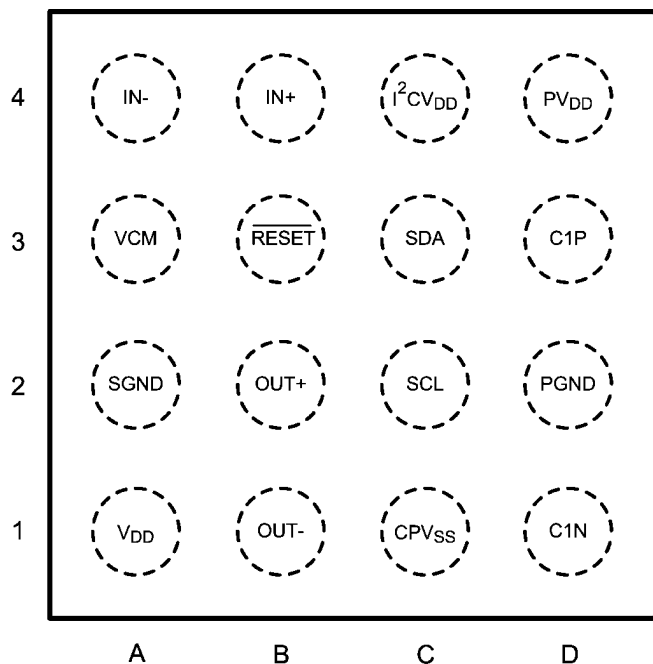
TL Package 1.965mm x 1.965mm x 0.6mm
