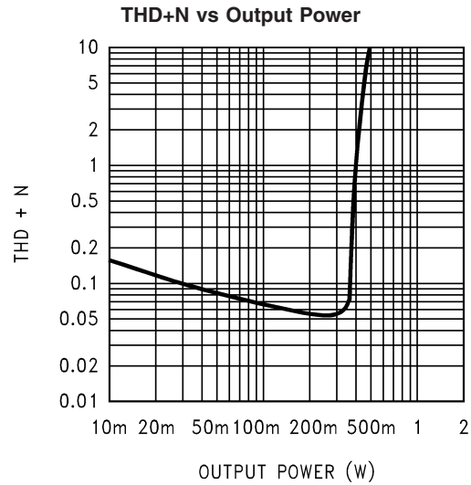
20106121 V_{DD} = 3V ; LLS, RLS; f = 1kHz ; R_L = 8\Omega ; Mode 7; 0dB Gain
