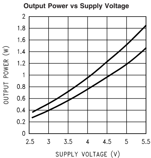
LLS, RLS; R_L = 8\Omega ; Top-10% THD+N; Bot-1% THD+N
