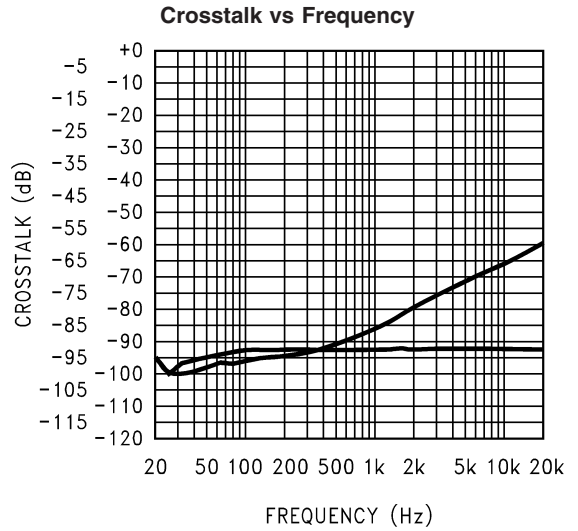
20106137 V DD = 3V; LHP, RHP; P O = 10mW; R L = 32Ω; Mode 9; 0db Gain; 3D off Top-Left to Right; Bot- Right to Left
