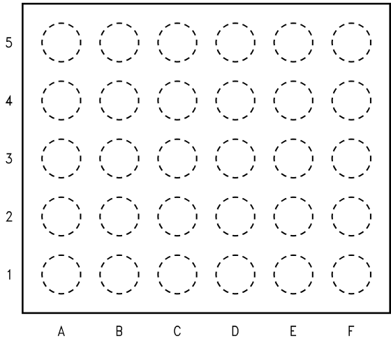
30 Bump ITL Package
