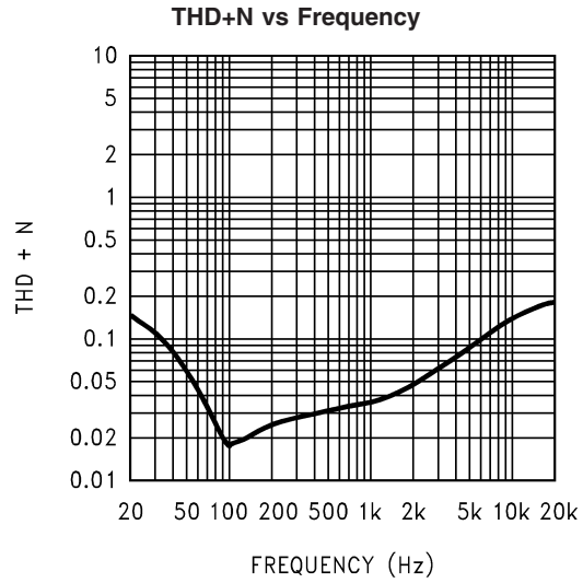
20106113 V_{DD} = 3V ; LHP, RHP; P_O = 10mW ; R_L = 32\Omega ; Mode 9; 0dB Gain
