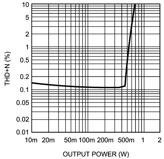
LM4859SP THD+N vs Output Power
