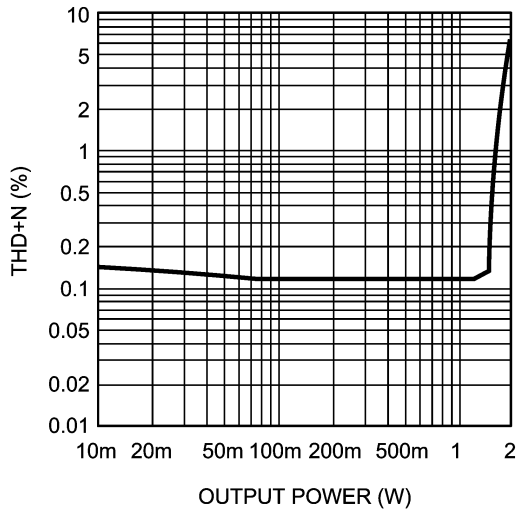
LM4859SP THD+N vs Output Power
