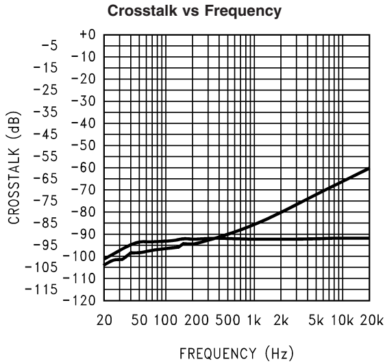
20106136 V DD = 5V; LHP, RHP; P O = 15mW; R L = 32Ω; Mode 9; 0db Gain; 3D off Top-Left to Right; Bot- Right to Left
