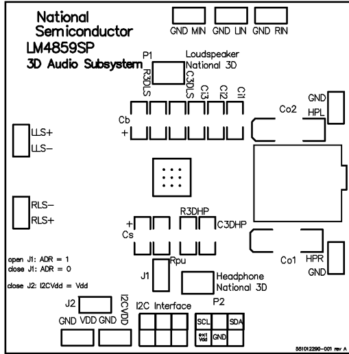
Recommended SP PCB Layout: Silkscreen Layer
