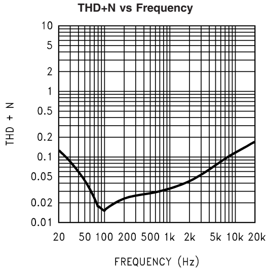
20106112 V_{DD} = 5V ; LHP, RHP; P_O = 15mW ; R_L = 32\Omega ; Mode 9; 0dB Gain
