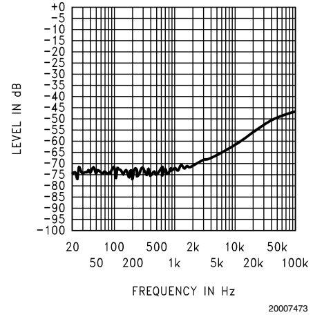
Input Floating
