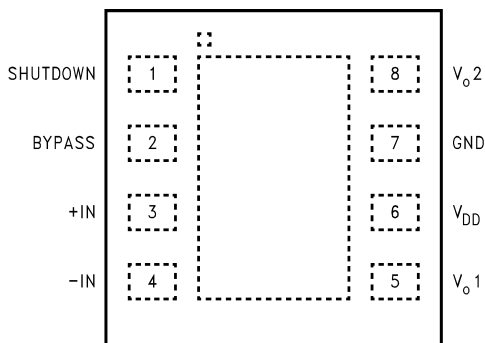
WSON Package (Top View) Package Number NGL
