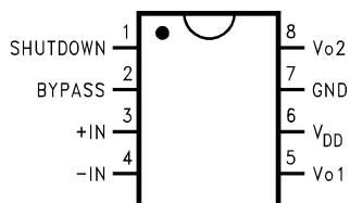
VSSOP and SOIC Package (Top View) Package Number DGK, D
