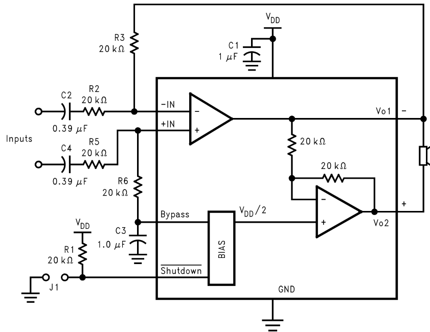
Figure 47. Differential Amplifier Configuration for LM4900
