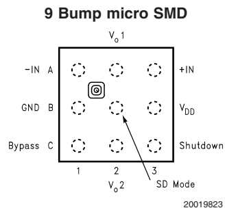
Top View Order Number LM4901IBL, LM4901IBLX See NS Package Number BLA09AAC
