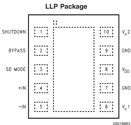
Top View Order Number LM4901LD See NS Package Number LDA10B
