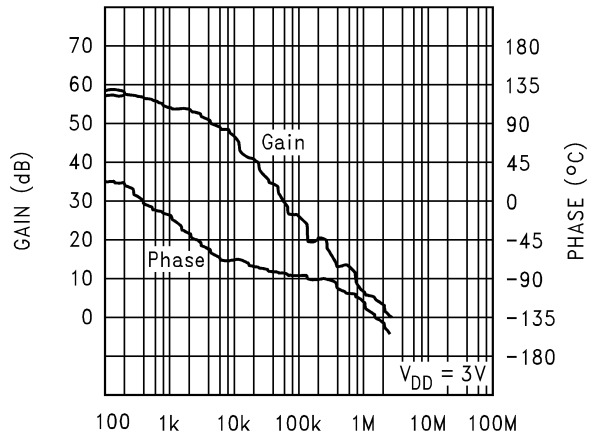
Open Loop Frequency Response, 3V
