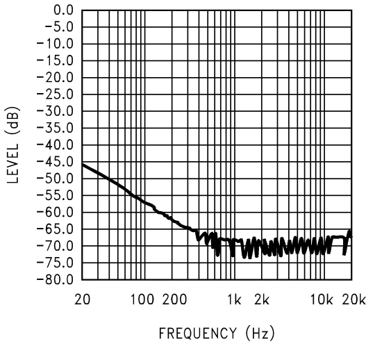
Input terminated with 10\Omega
