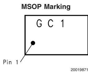
Top View G - Boomer Family C1 - LM4901MM
