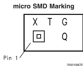
Top View X - Date Code T - Die Traceability G - Boomer Family Q - LM4901IBL
