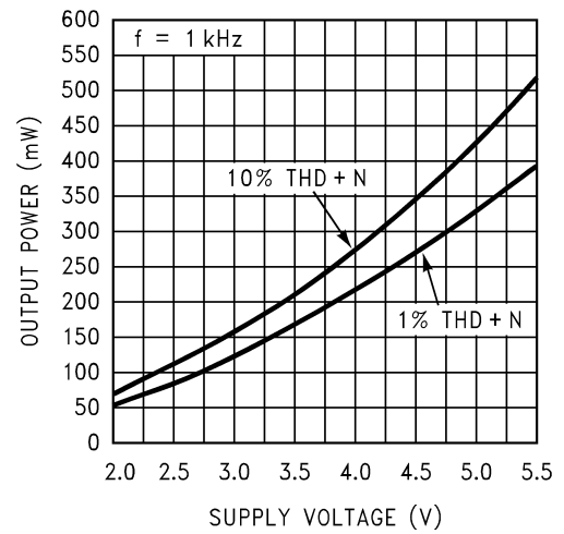
Output Power vs Supply Voltage, 32Ω
