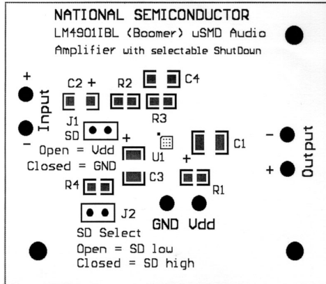
Silk Screen
