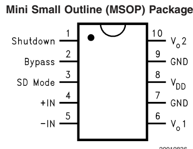
Top View Order Number LM4901MM See NS Package Number MUB10A
