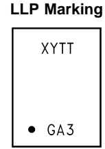
Top View XY - Date Code TT - Die Traceability G - Boomer Family A3 - LM4902LD
