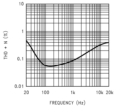
THD+N vs Frequency at V_{DD} = 3V , 8\Omega R_L , and PWR = 250mW
