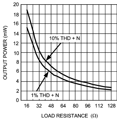
Output Power vs Load Resistance V_{DD} = 1.5V, R_L = 16\Omega, f = 1kHz Single Ended Output, A_V = -1
