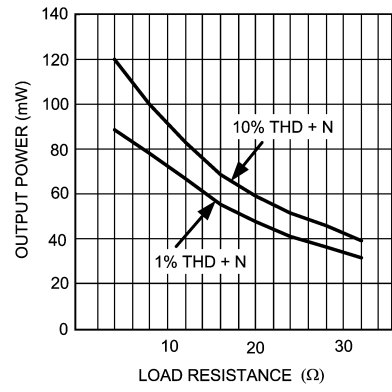
Output Power vs Load Resistance V_{DD} = 1.5V, R_L = 8\Omega, f = 1kHz BTL Output, A_V = -1
