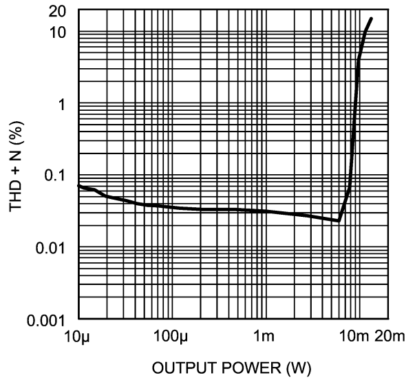
THD+N vs Output Power V_{DD} = 1.6V, R_L = 32\Omega, f = 1kHz One channel enabled
