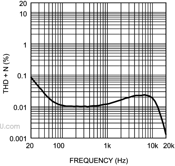
THD+N vs Frequency V_{DD} = 4.2V, R_L = 16\Omega, P_O = 150mW
