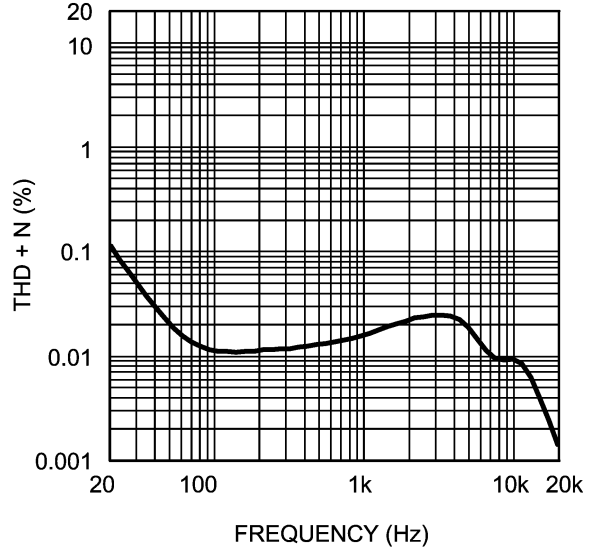
THD+N vs Frequency V_{DD} = 4.2V, R_L = 32\Omega, P_O = 150mW
