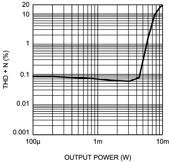
THD+N vs Output Power V_{DD} = 1.6V, R_L = 16\Omega, f = 1kHz One channel enabled
