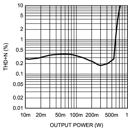
THD+N vs Output Power ( A_{V_{DD}} = 3.3V , R_L = 8\Omega , f = 1kHz , Handsfree Output)
