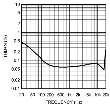
THD+N vs Frequency ( A_{V_{DD}} = 3.3V , R_L = 32\Omega , P_O = 7.5mW , Headphone Output)
