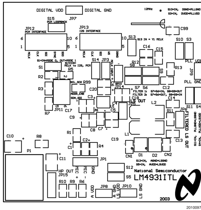
FIGURE 10. LM4931ITL Demo Board Silkscreen
