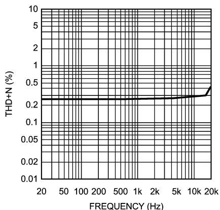
THD+N vs Frequency ( A_{V_{DD}} = 3.3V , R_L = 8\Omega , P_O = 200mW , Handsfree Output)
