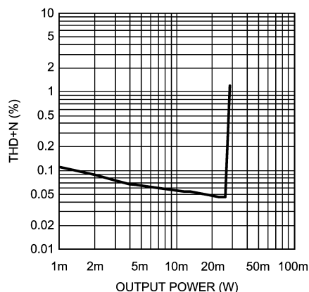
THD+N vs Output Power ( A_{V_{DD}} = 3V , R_L = 32\Omega , f = 1kHz , Headphone Output)
