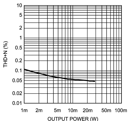
THD+N vs Output Power ( A_{V_{DD}} = 5V , R_L = 32\Omega , f = 1kHz , Headphone Output)
