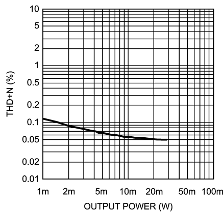
THD+N vs Output Power ( A_{V_{DD}} = 3.3V , R_L = 32\Omega , f = 1kHz , Headphone Output)
