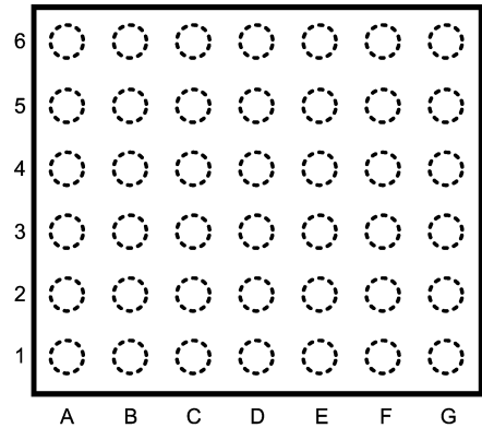
42-Bump Microfil
