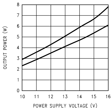
200756E8 R_L = 4\Omega , SE operation, both channels driven and loaded (average shown), at (from top to bottom at 12V): THD+N = 10%, THD+N = 1%
