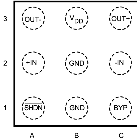
9 Bump micro SMD Package
