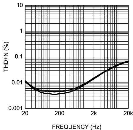
THD+N vs Frequency V_{DD} = 3.3V , R_L = 32\Omega , P_O = 12mW Mode 4, 7, OCL, BW = 80kHz
