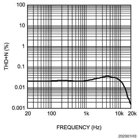
THD+N vs Frequency OCL Headphone Mode, Single-Ended Input V_{DD} = 5.0V, P_{OUT} = 50mW, R_L = 32\Omega
