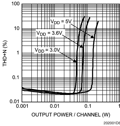
THD+N vs Output Power CC Headphone Mode, Single-Ended Input A_V = 0\text{dB} , R_L = 16\Omega , f = 1\text{kHz}
