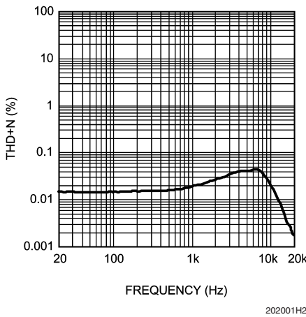
THD+N vs Frequency OCL Headphone Mode, Single-Ended Input V_{DD} = 3.6V, P_{OUT} = 30mW, R_L = 32\Omega
