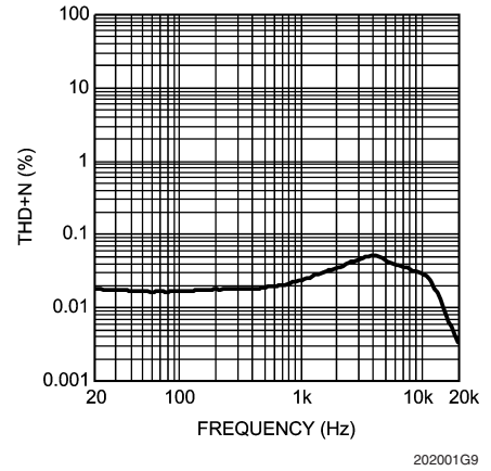
THD+N vs Frequency OCL Headphone Mode, Single-Ended Input V_{DD} = 3.0V, P_{OUT} = 20mW, R_L = 32\Omega
