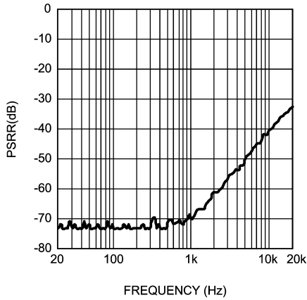
PSRR vs Frequency CC Headphone Mode, Differential Input V_{DD} = 3.6V , V_{RIPPLE} = 200mV_{P-P} , R_L = 32\Omega
