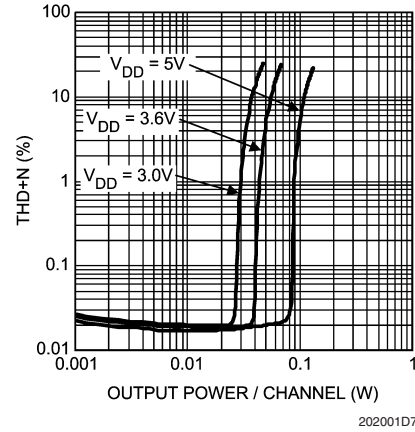
THD+N vs Output Power CC Headphone Mode, Differential Input A_V = 0\text{dB} , R_L = 32\Omega , f = 1\text{kHz}
