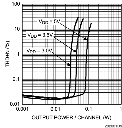
THD+N vs Output Power CC Headphone Mode, Single-Ended Input A_V = 0\text{dB} , R_L = 32\Omega , f = 1\text{kHz}
