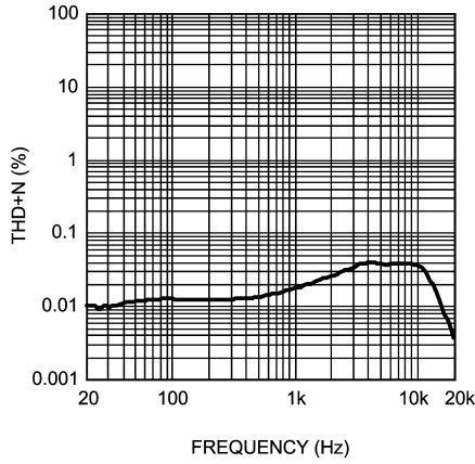
THD+N vs Frequency CC Headphone Mode, Single-Ended Input V_{DD} = 3.0V, P_{OUT} = 35mW, R_L = 16\Omega
