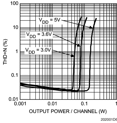
THD+N vs Output Power CC Headphone Mode, Differential Input A_V = 0\text{dB} , R_L = 16\Omega , f = 1\text{kHz}
