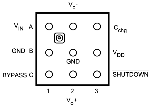
Top View Order Number LM4951TL, TLX See NS Package Number TLA09ZZA
