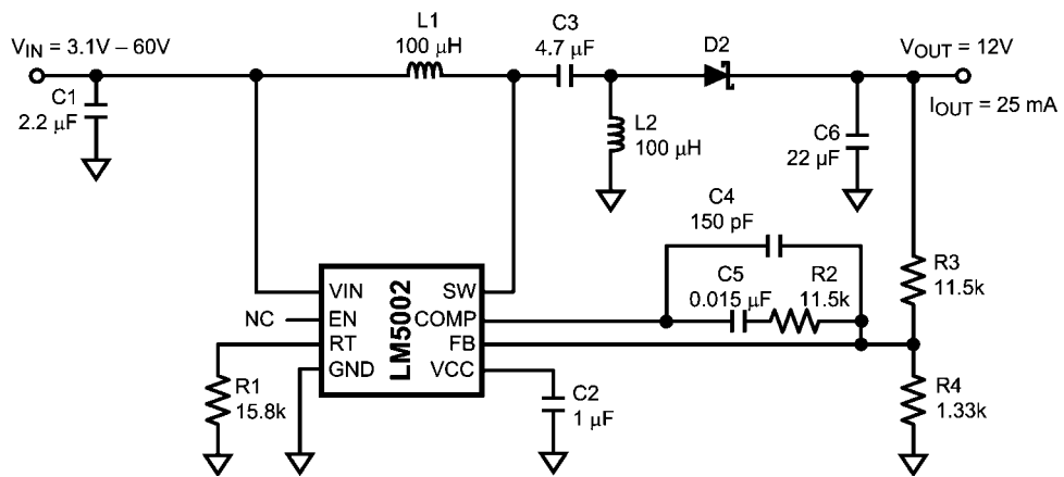
FIGURE 10. 12V SEPIC
