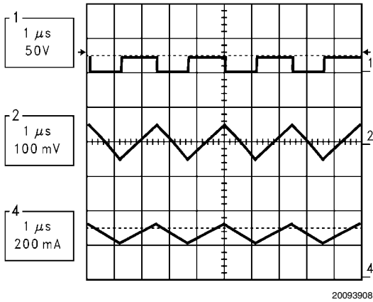
Operational Waveforms
