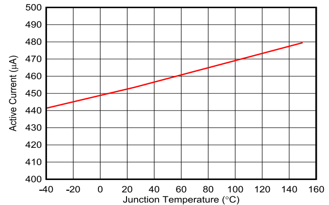
Figure 7-4. VIN Active Current Versus Temperature
