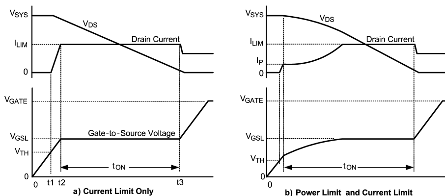
FIGURE 11. MOSFET Power Up Waveforms
