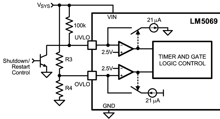
FIGURE 14. UVLO = \text{POR}_{\text{EN}} with Shutdown/Restart Control
