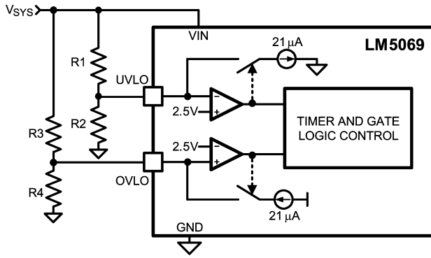
FIGURE 13. Programming the Four Thresholds
