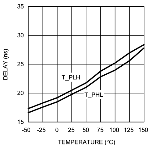
LM5100A/B/C Propagation Delay vs Temperature
