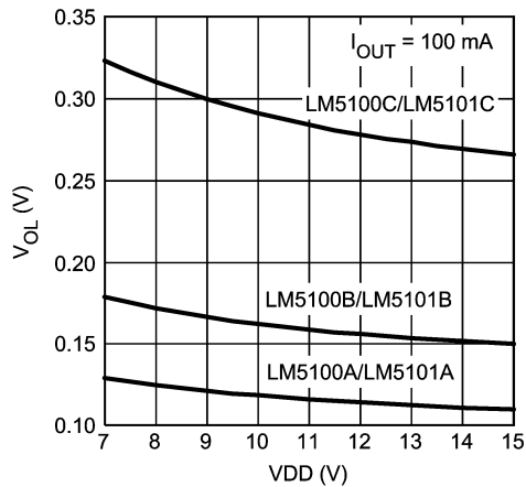
LO & HO Gate Drive - Output Low Voltage vs VDD
