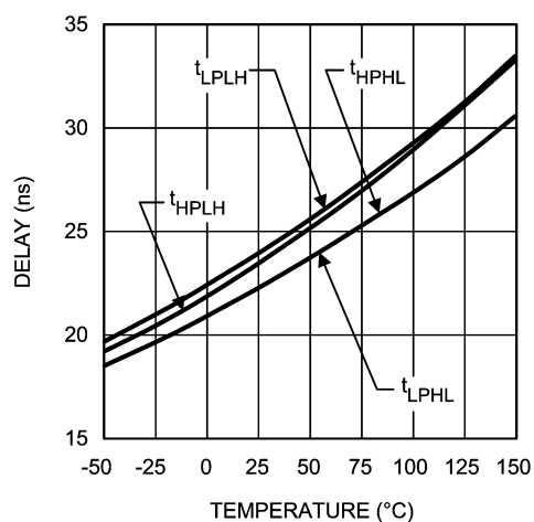
LM5100 Propagation Delay vs Temperature
