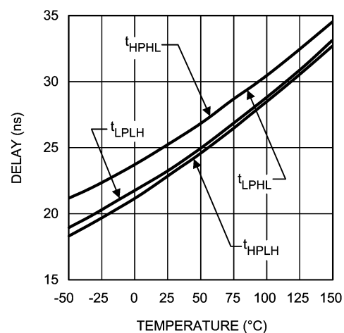
LM5101 Propagation Delay vs Temperature
