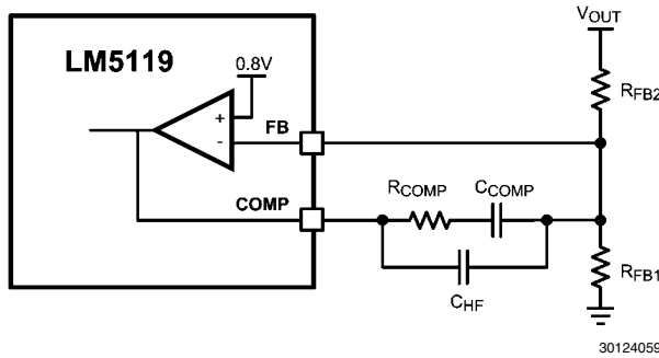
FIGURE 7. Feedback Configuration
