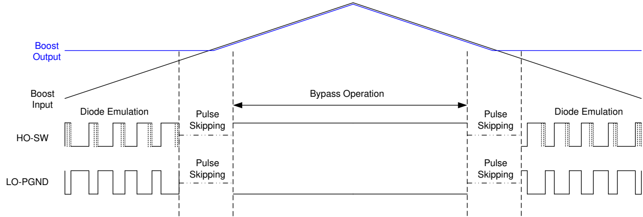
Figure 8-18. PWM to Bypass Transition in DCM Operation
