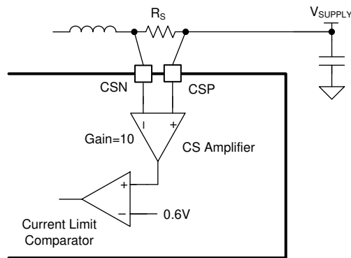
Figure 8-15. Current Limit Comparator
