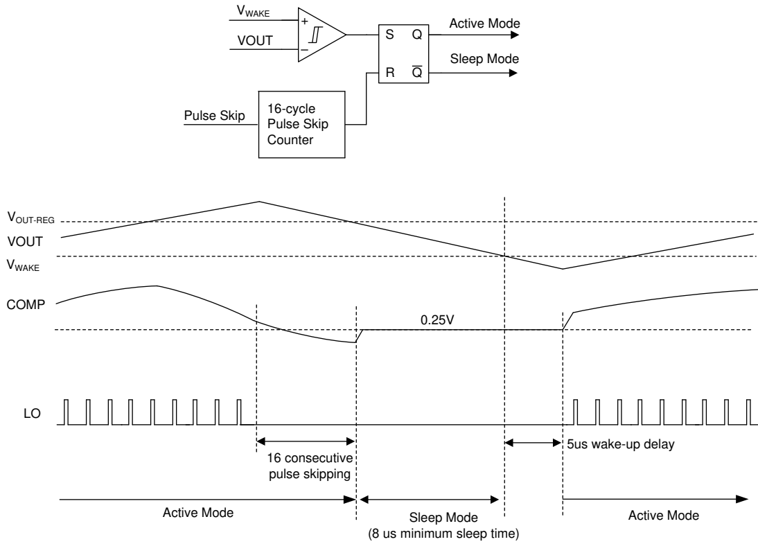
Figure 8-23. Skip Mode Operation
