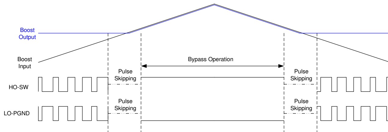
Figure 8-17. PWM to Bypass Transition in CCM Operation
