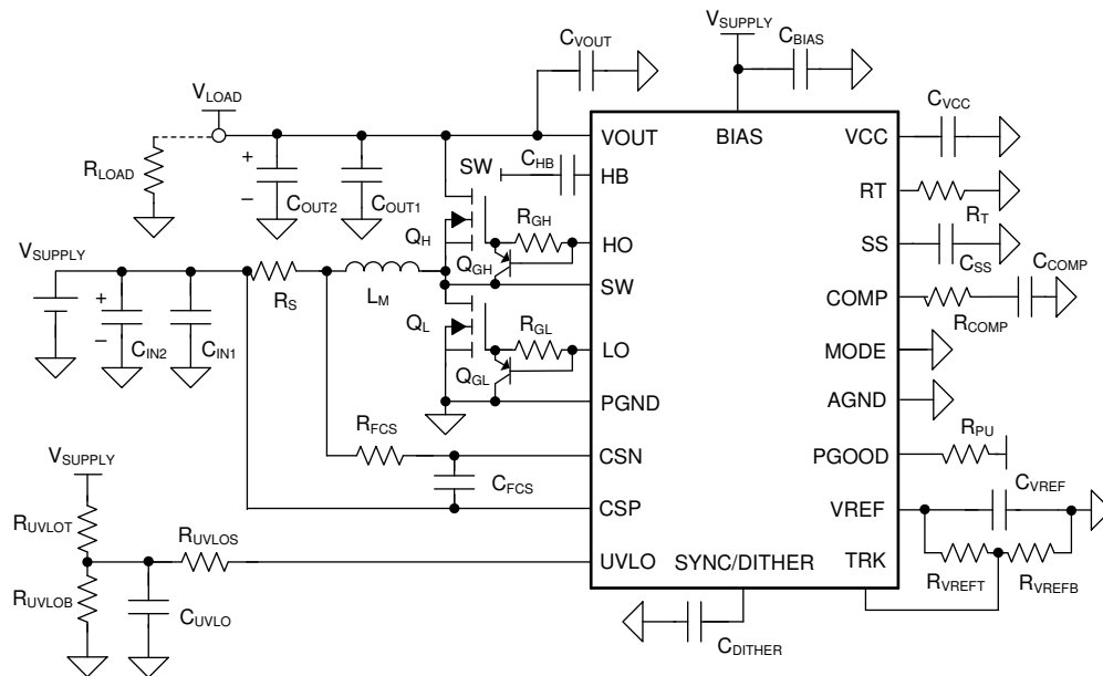
Figure 9-1. Typical Synchronous Boost Converter with Optional Components
