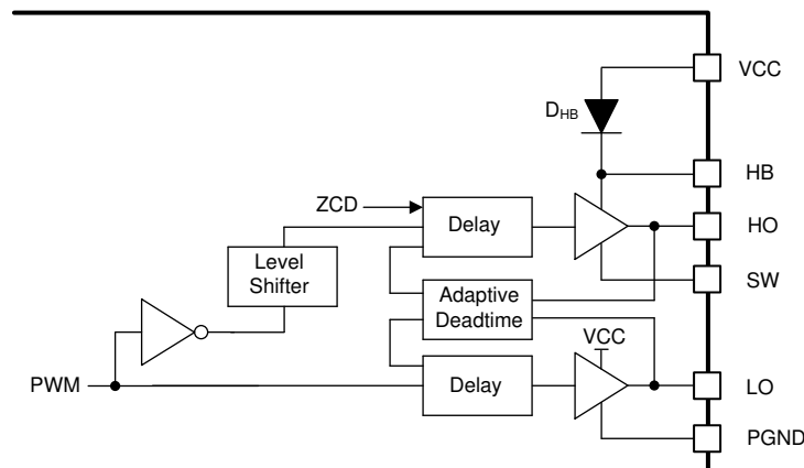
Figure 8-19. Driver Structure with Internal Boot Diode
