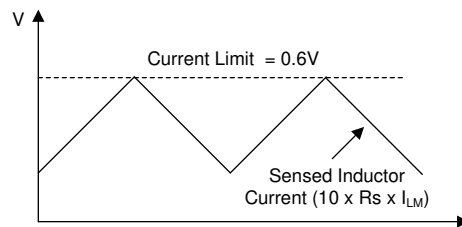
Figure 8-16. Current Limit Comparator Input
