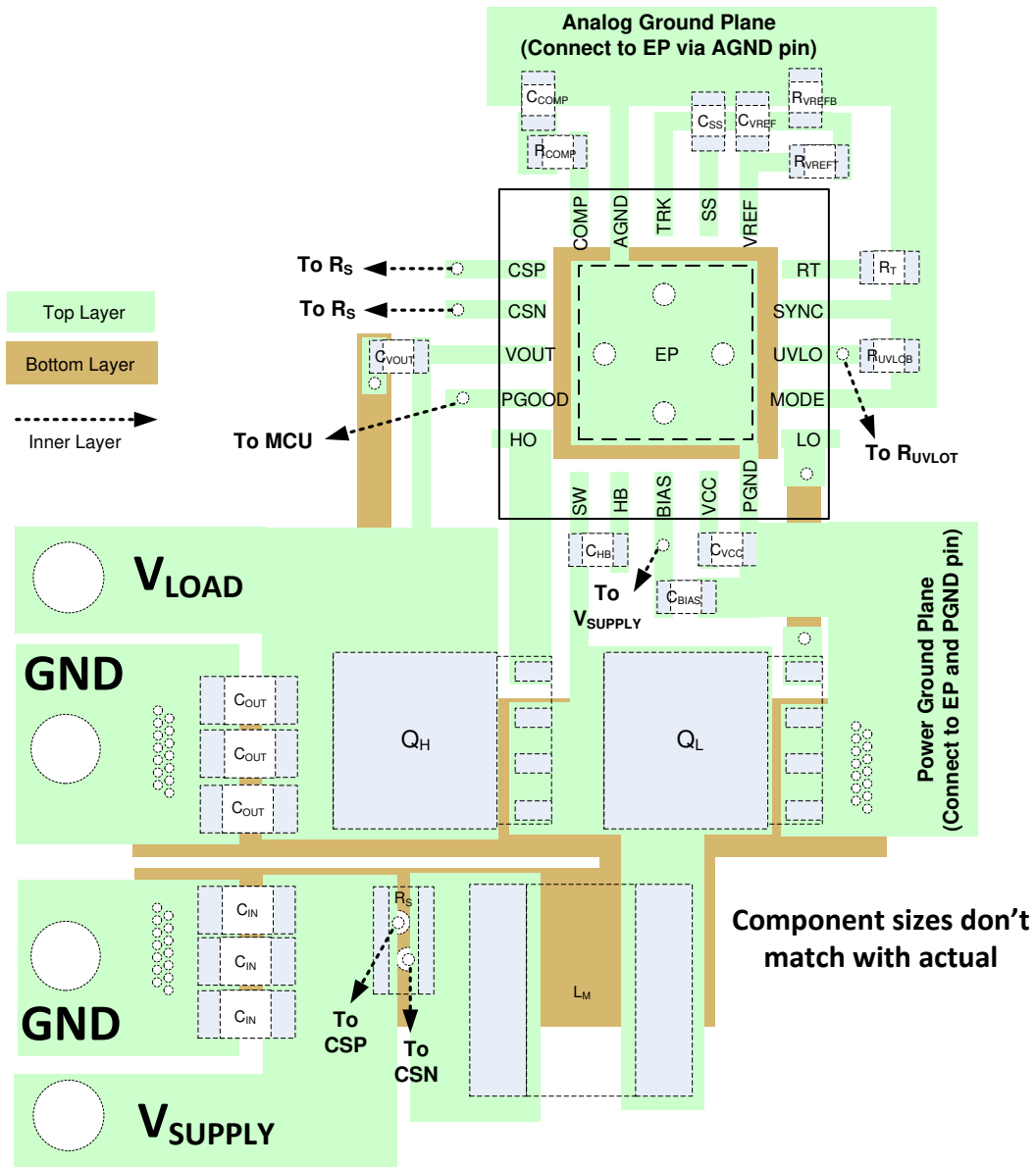
Figure 11-1. PCB Layout Example
