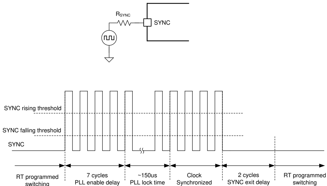
Figure 8-9. External Clock Synchronization
