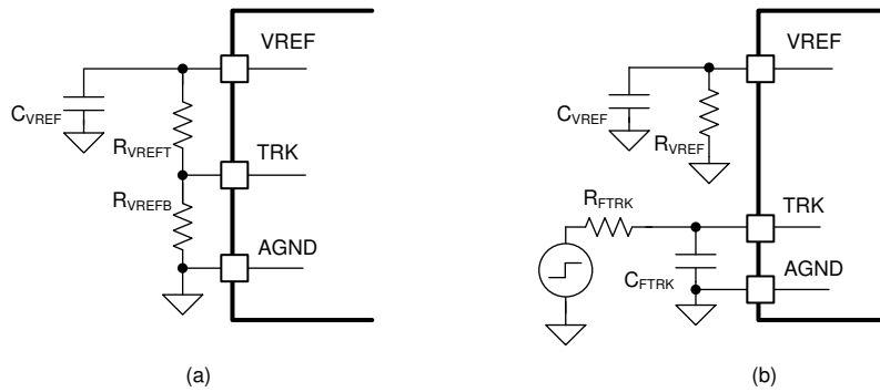
Figure 8-6. TRK Control (a) using VREF (b) by External Step Input
