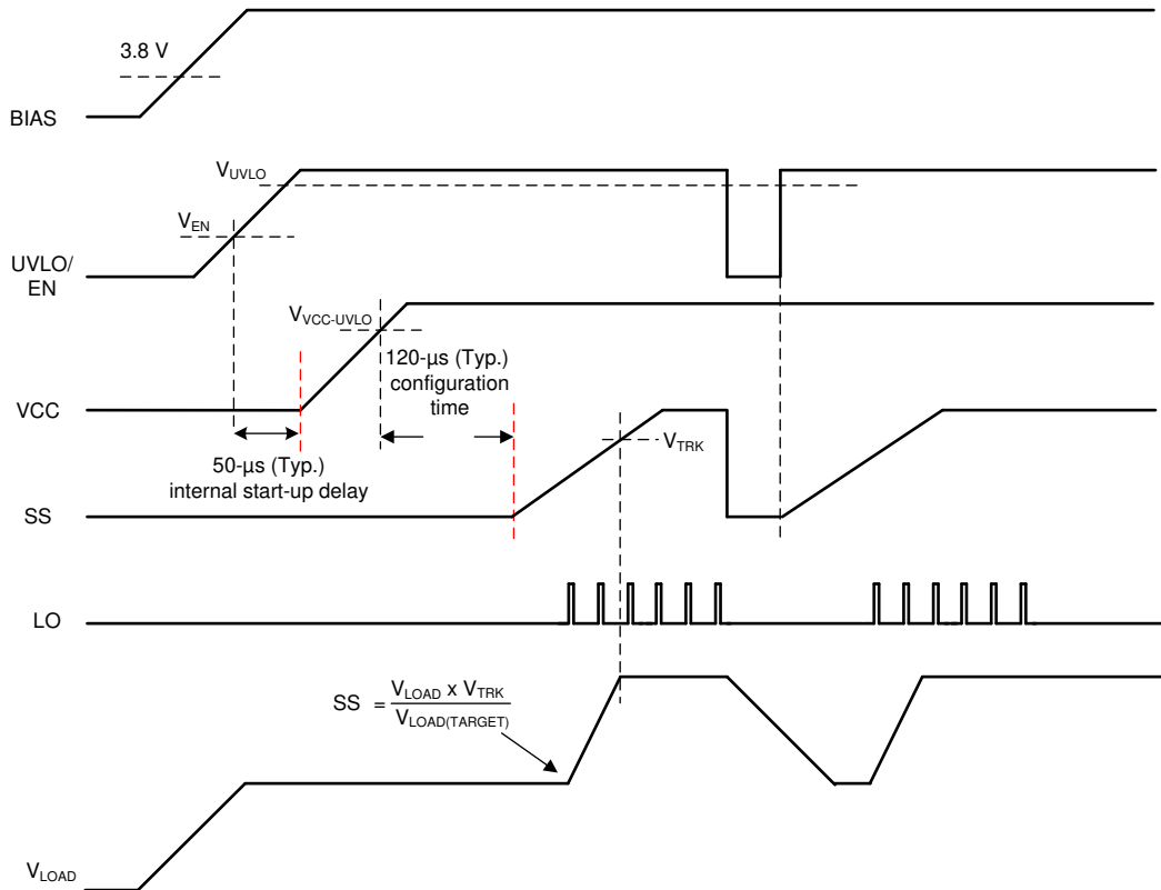
Figure 8-5. Boost Start-up Waveforms Case 2: Start-up by EN/UVLO, Restart when V_H > V_{SYNC}
