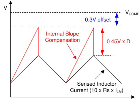
Figure 8-14. PWM Comparator Input
