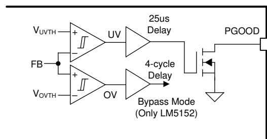
Figure 8-7. PGOOD Indicator
