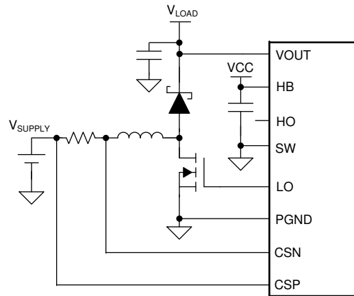
Figure 9-4. Non-synchronous Boost Configuration
