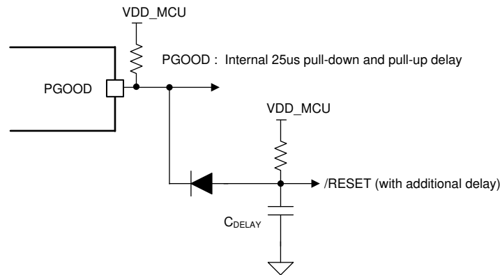
Figure 9-3. Additional PGOOD Delay
