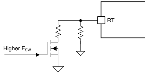
Figure 8-8. Frequency Hopping Example
