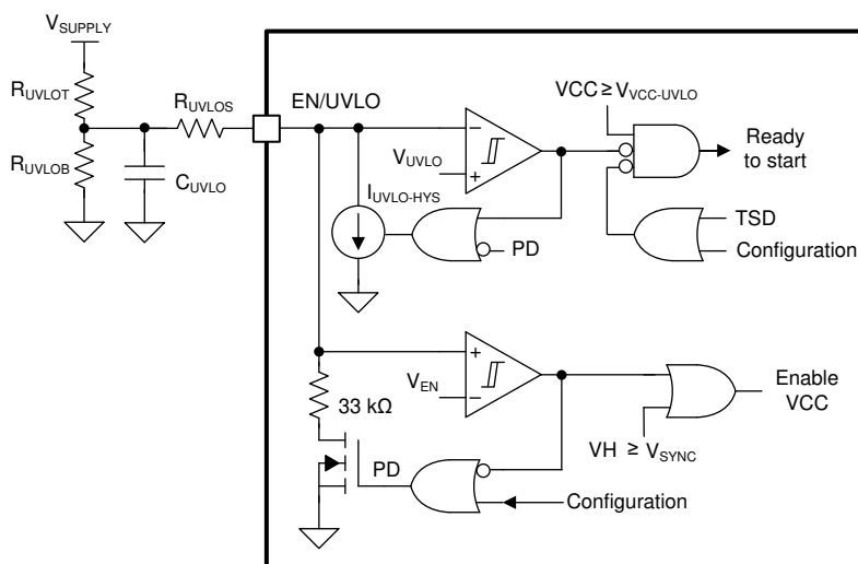
Figure 8-1. EN/UVLO Circuit
