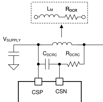
Figure 9-2. DCR Current Sensing
