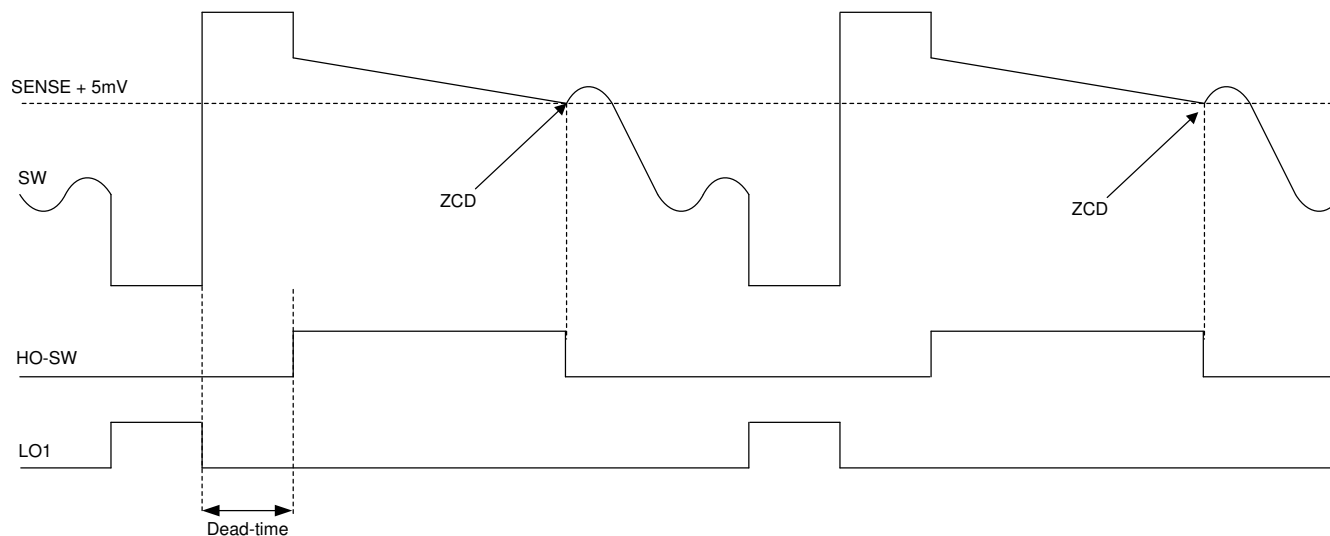
Figure 8-22. Zero Current Detection
