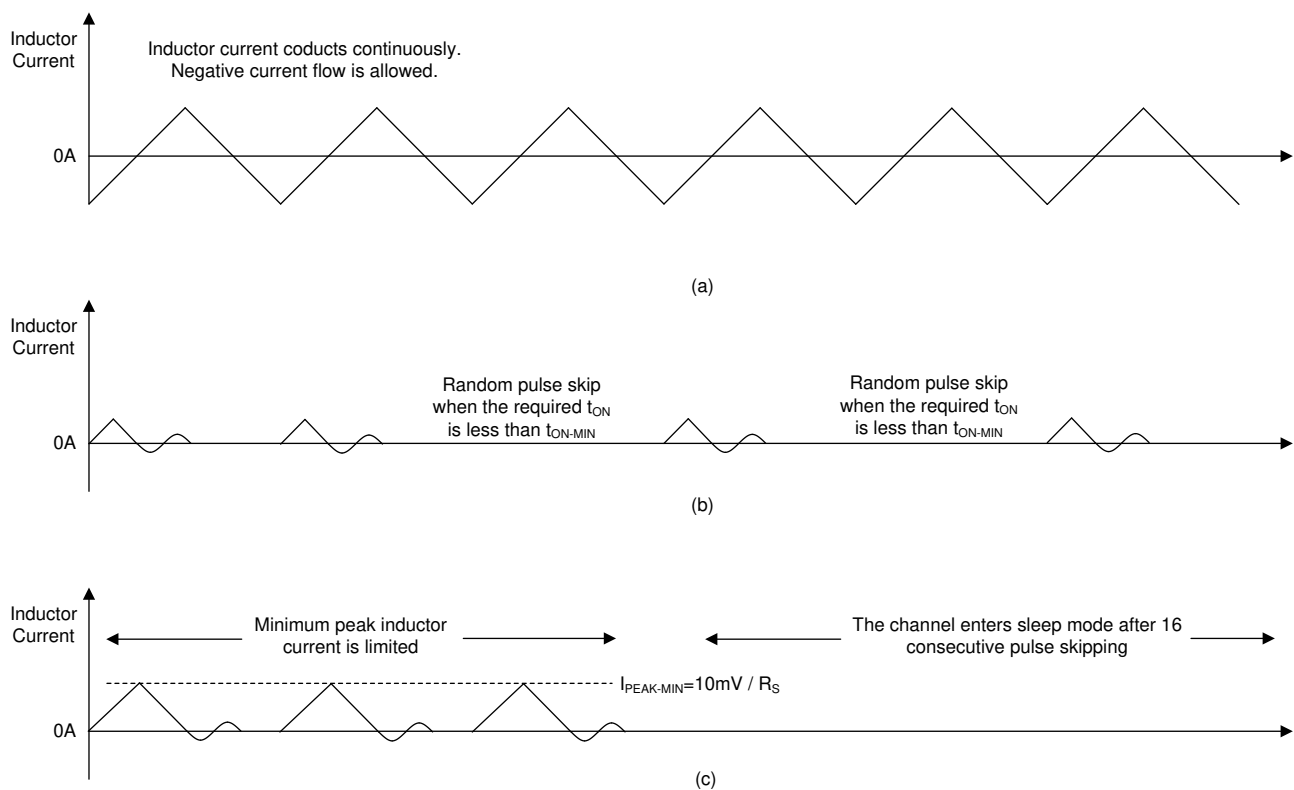
Figure 8-21. Inductor Current Waveform at Light Load (a) FPWM (b) Diode Emulation (c) Skip Mode
