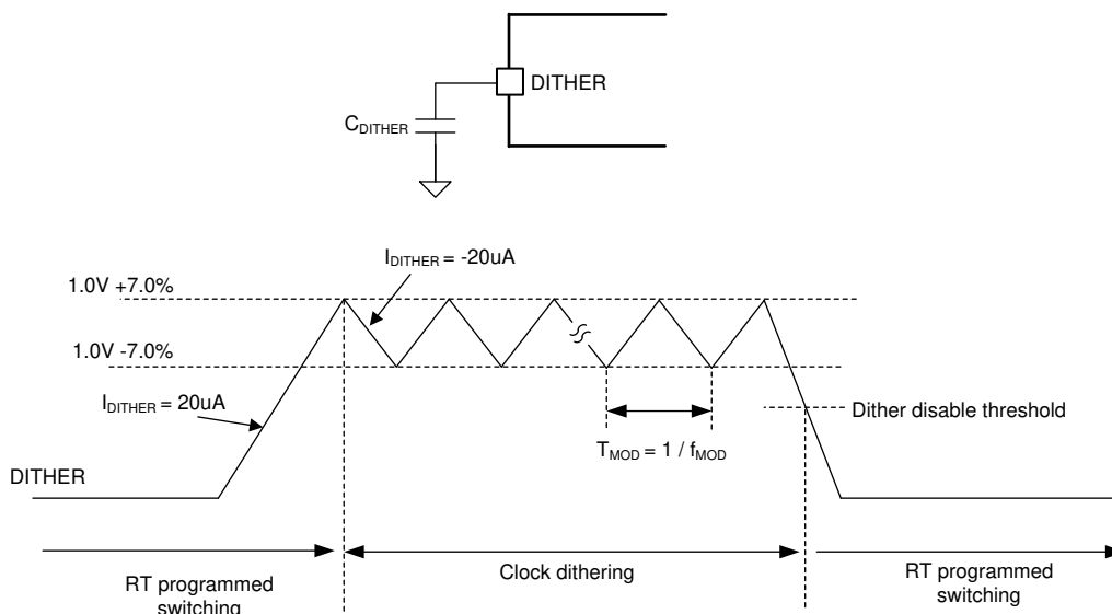
Figure 8-10. Switching Frequency Dithering
