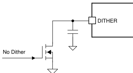
Figure 8-11. Dynamic Dither On/Off Example
