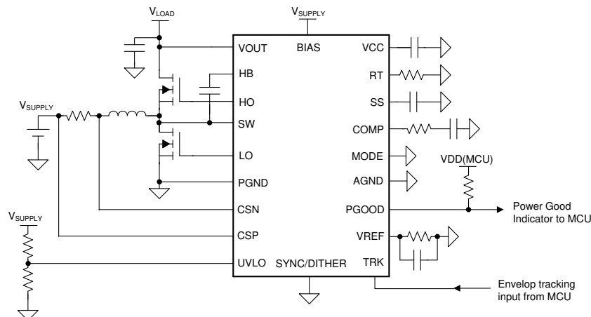
Typical Application
