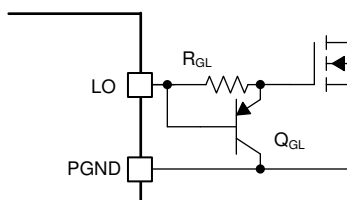
Figure 8-20. Slew Rate Control
