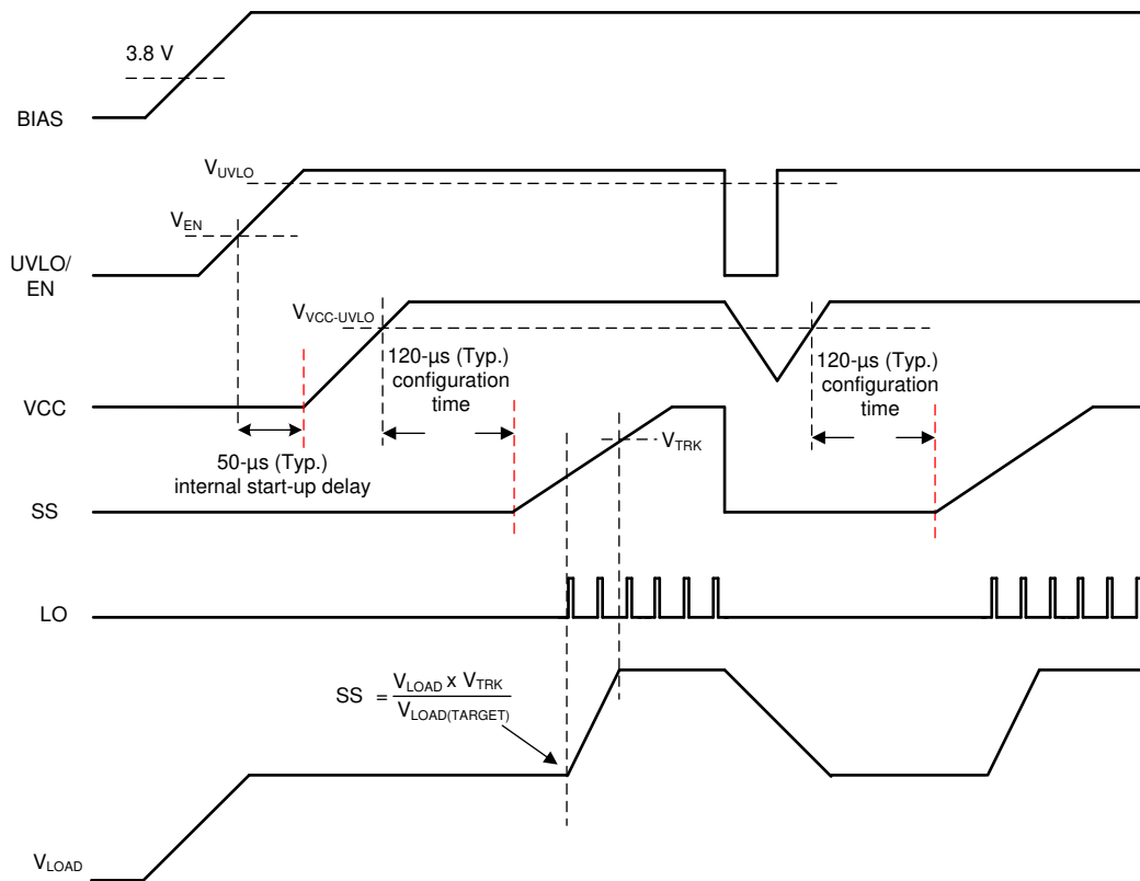
Figure 8-4. Boost Start-up Waveforms Case 1: Start-up by EN/UVLO, Restart when V_H < V_{SYNC}
