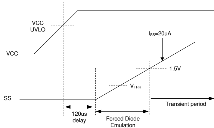
Figure 8-12. Soft Start and Smooth Transition to FPWM
