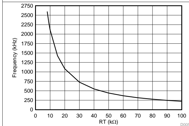
Figure 5. Frequency vs R_T
