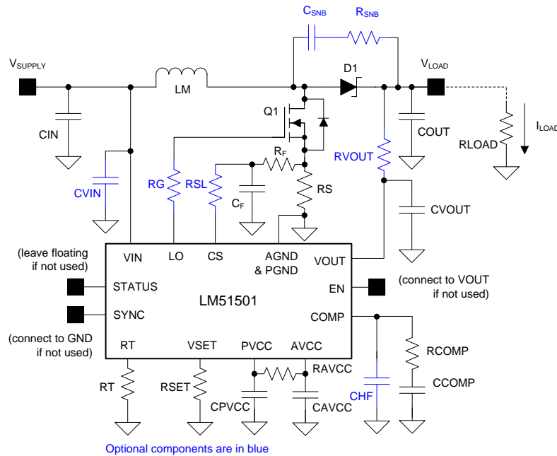
Figure 19. Typical Circuit With Optional Components
