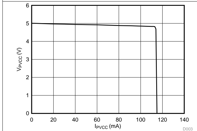
Figure 3. V_{PVCC} vs I_{PVCC} ( V_{OUT} = 6 \text{ V} )
