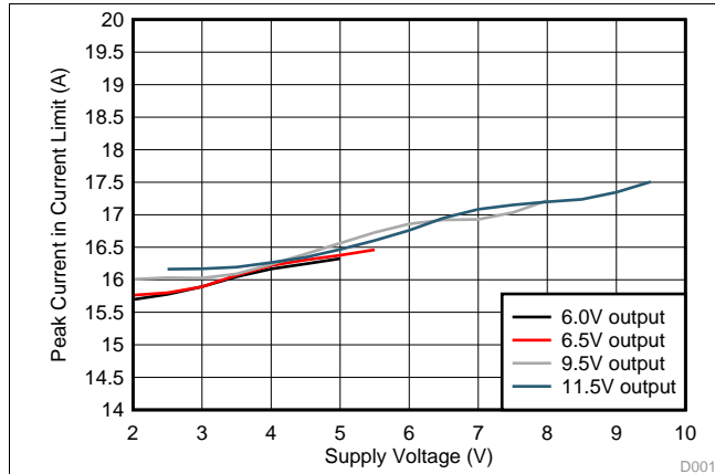
Figure 1. Peak Inductor Current vs Supply Voltage ( F_{sw} = 440 \text{ kHz} , R_S = 7 \text{ m}\Omega , R_F = 100 \text{ }\Omega , C_F = 2.2 \text{ nF} )
