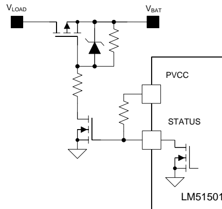
Figure 18. Disconnection Switch Control Example
