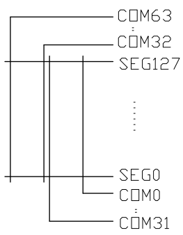
Wiring Details (Top View) Scale=free.
