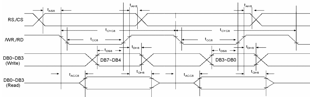
Bus Timing Diagram
