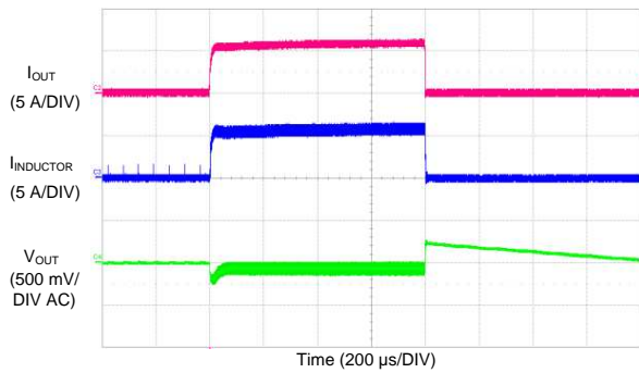
Figure 81. LM73606-Q1 Load Transients
