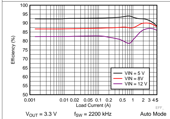
Figure 31. LM73605-Q1 Efficiency
