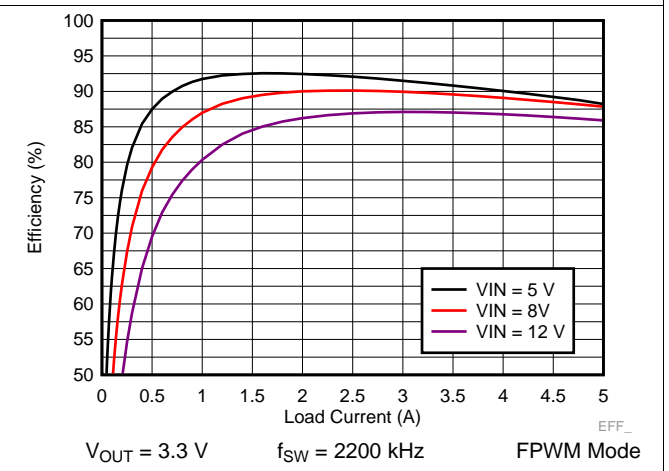
Figure 32. LM73605-Q1 Efficiency
