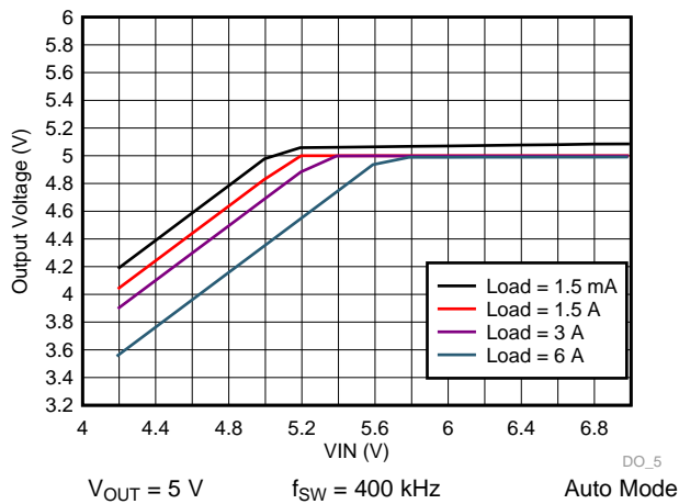
Figure 59. LM73606-Q1 Dropout Curve
